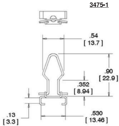
Plastic Connectors Mounted to Front of Panel
