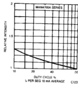
Fig. 14. Luminous Intensity vs. Duty Cycle
