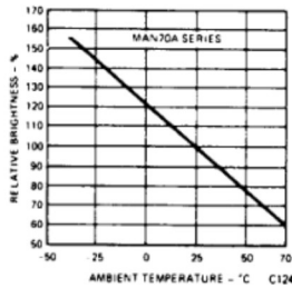
Fig. 7. Relative Luminous Intensity vs. Temperature
