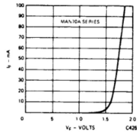
Fig. 6. Forward Current vs. Forward Voltage
