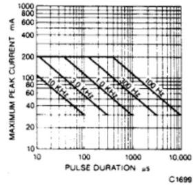
Fig. 10. Maximum Peak Current vs. Pulse Duration
