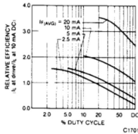
Fig. 11. Relative Efficiency vs. Duty Cycle
