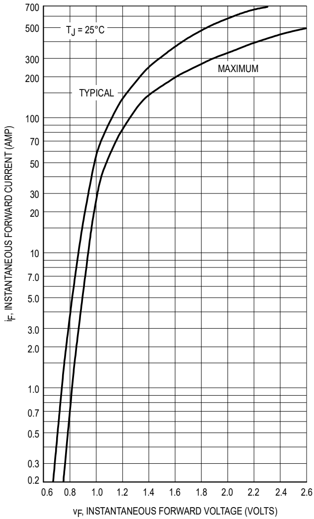
Figure 1. Forward Voltage
