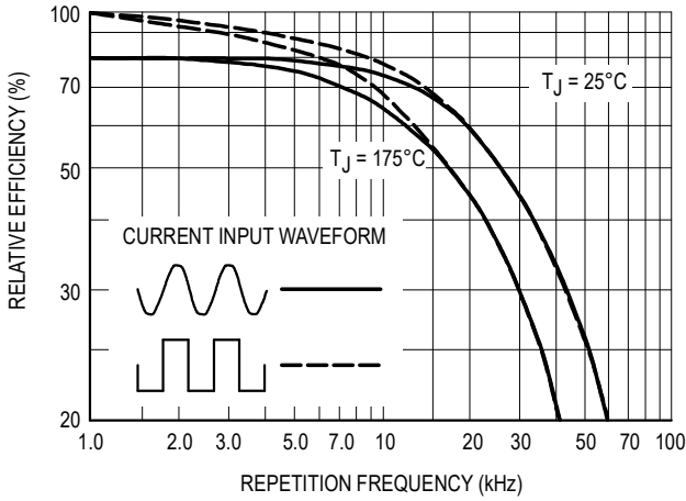
Figure 9. Rectification Efficiency
