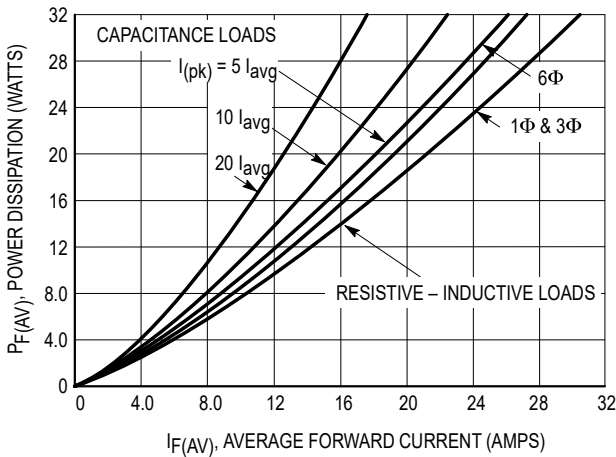
Figure 7. Power Dissipation
