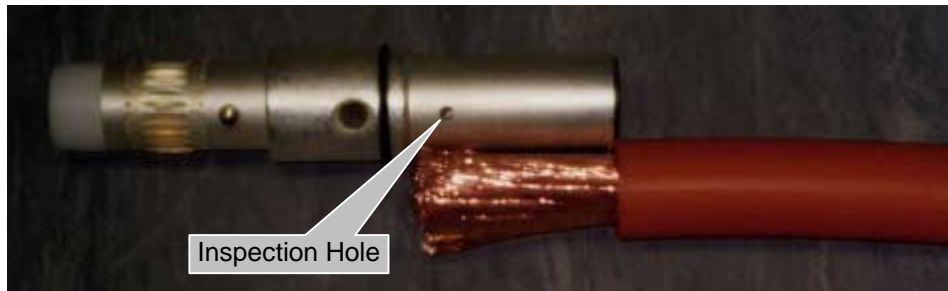
Figure 6. Inspection Hole In Contact
