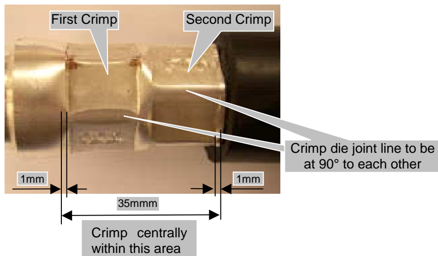
Figure 5. Recommended Double Crimp Arrangement
